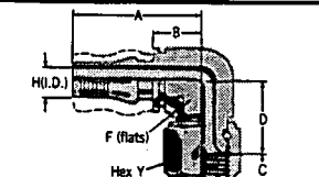
90° elbow forged
