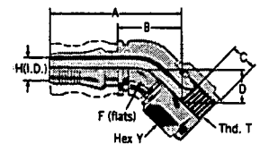
45° elbow forged
